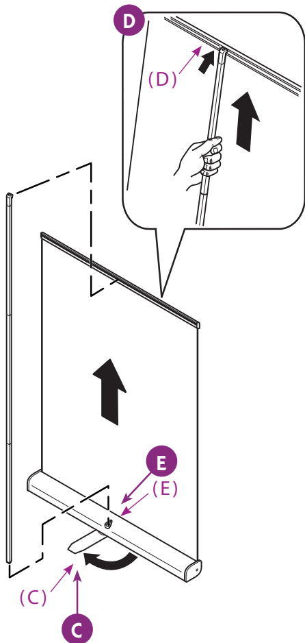
LOCKING MECHANISM
