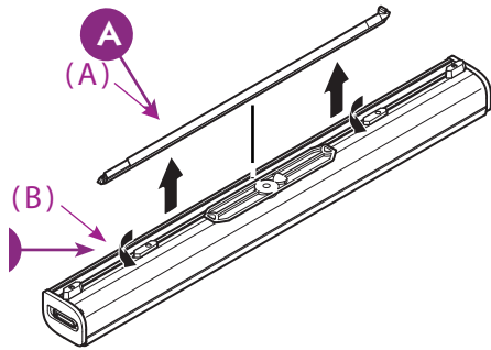
TIGHTENING SPRING (1)
